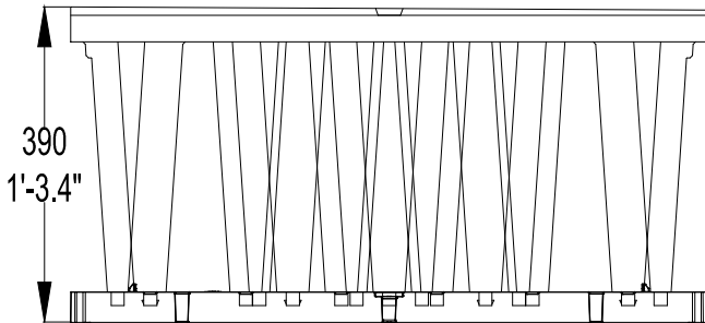
EcoBloc maxx system 402201 + 402200
